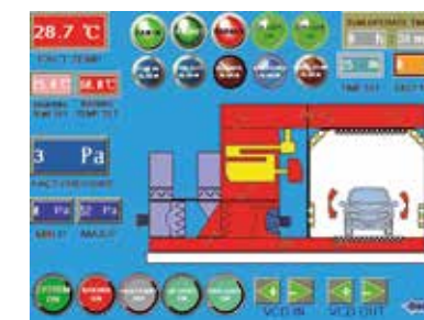
Touch-skärm / Drift
